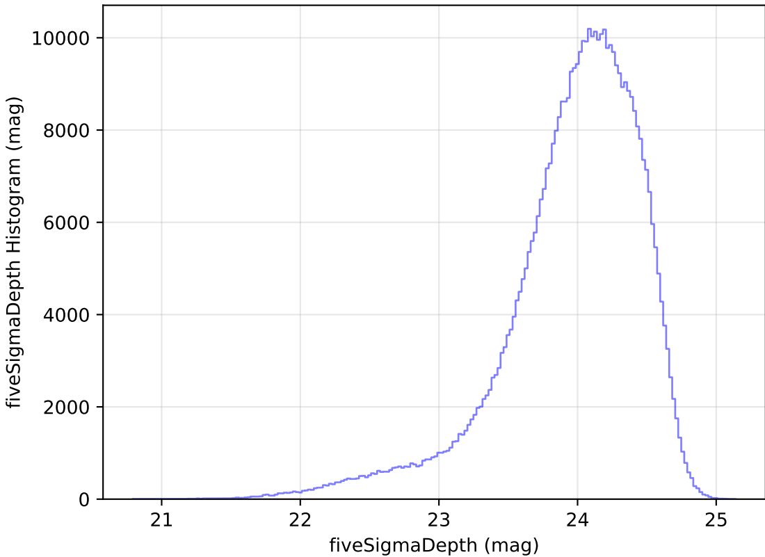
too_elab_r256_d3_griz_v3.4_10yrs r: fiveSigmaDepth Histogram
