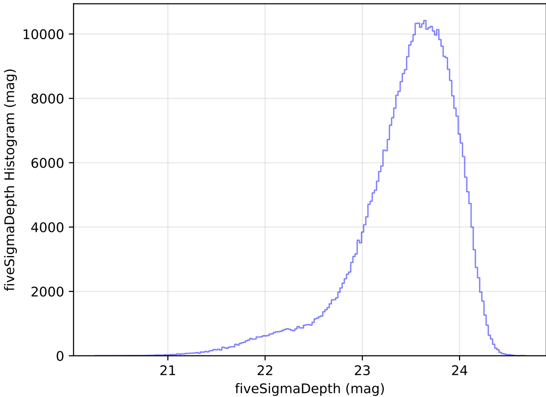
too_elab_r256_d3_griz_v3.4_10yrs i: fiveSigmaDepth Histogram
