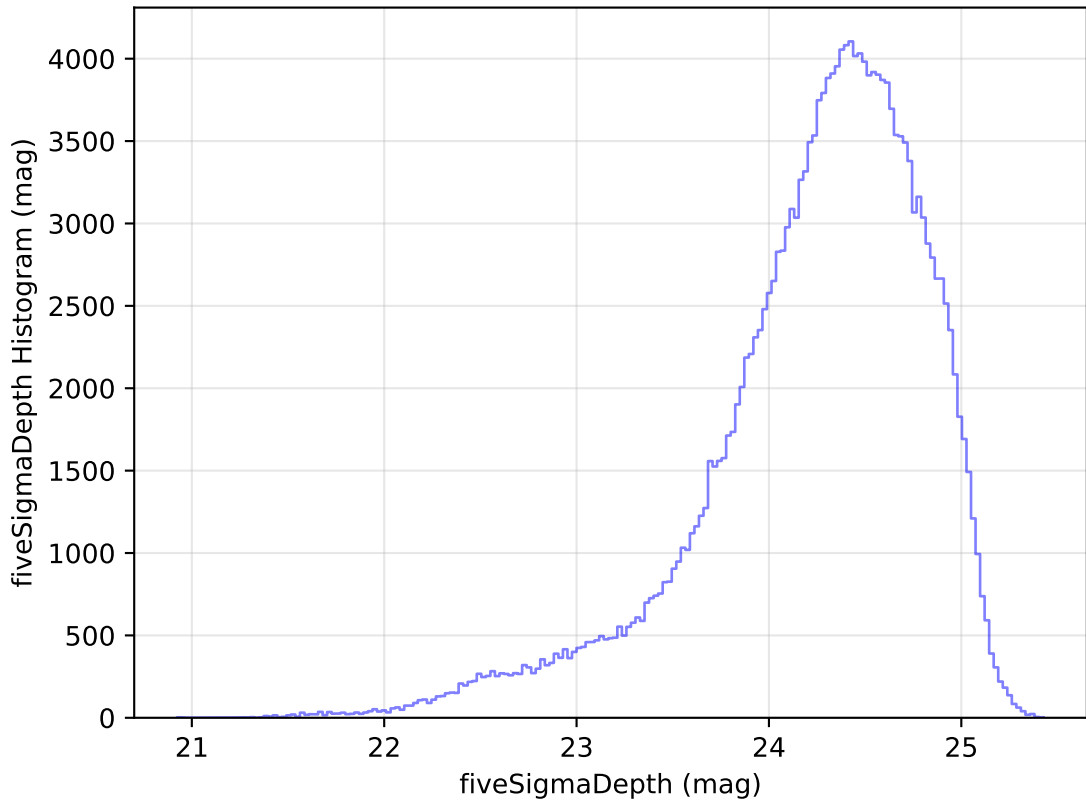
too_elab_r256_d3_griz_v3.4_10yrs g: fiveSigmaDepth Histogram
