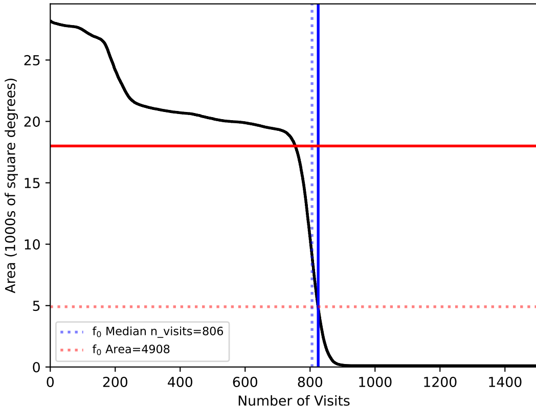
too_elab_r256_d3_griz_v3.4_10yrs : fO
