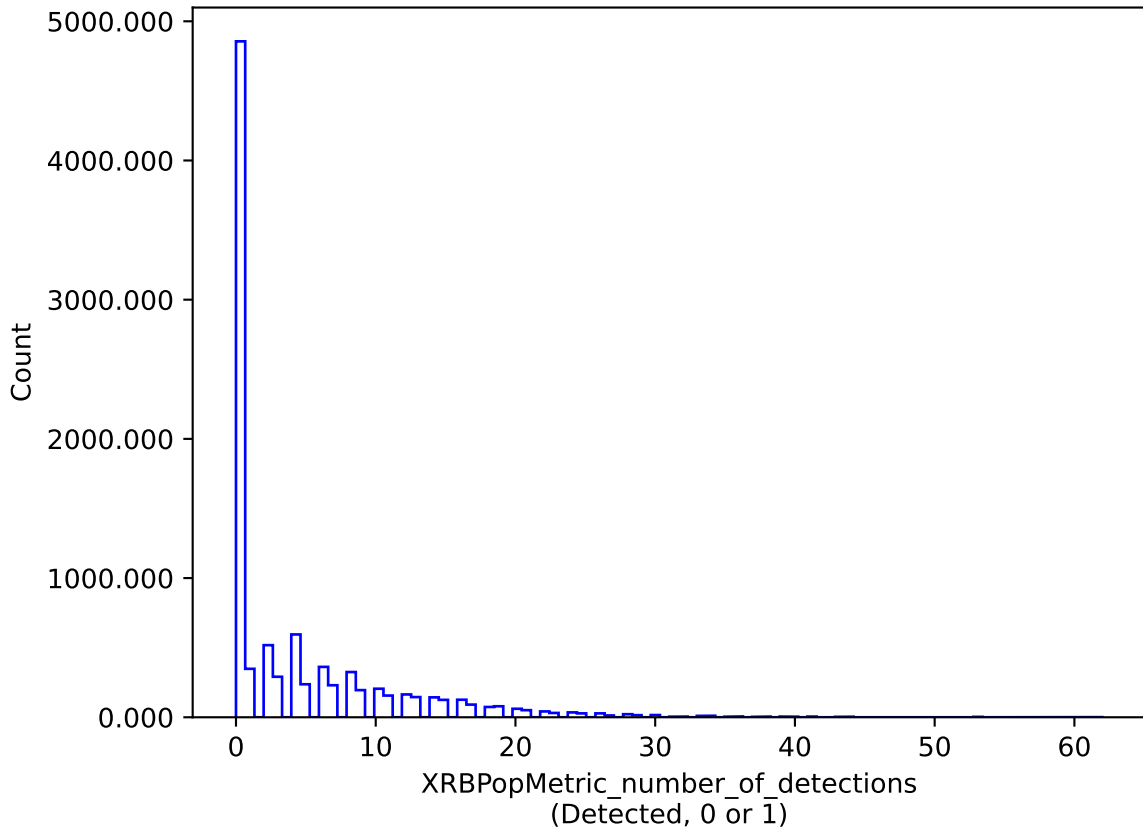
too_elab_r256_d3_griz_v3.4_10yrs : XRBPopMetric_number_of_detections
