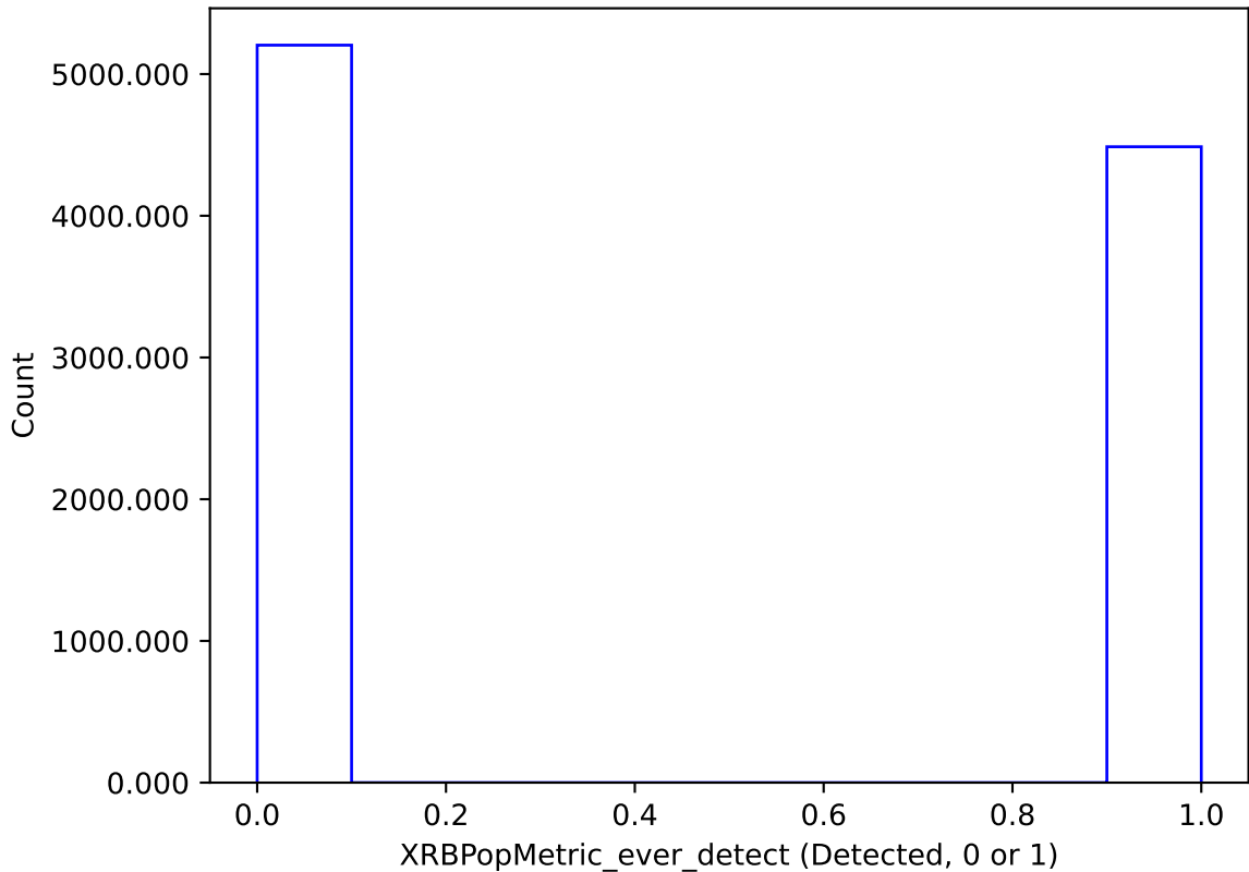
too_elab_r256_d3_griz_v3.4_10yrs : XRBPoMetric_ever_detect
