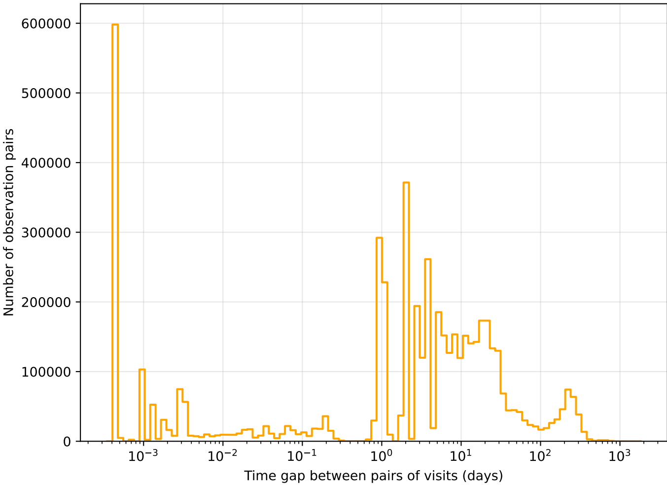
too_elab_r256_d3_griz_v3.4_10yrs r band: Tgaps observationStartMJD
