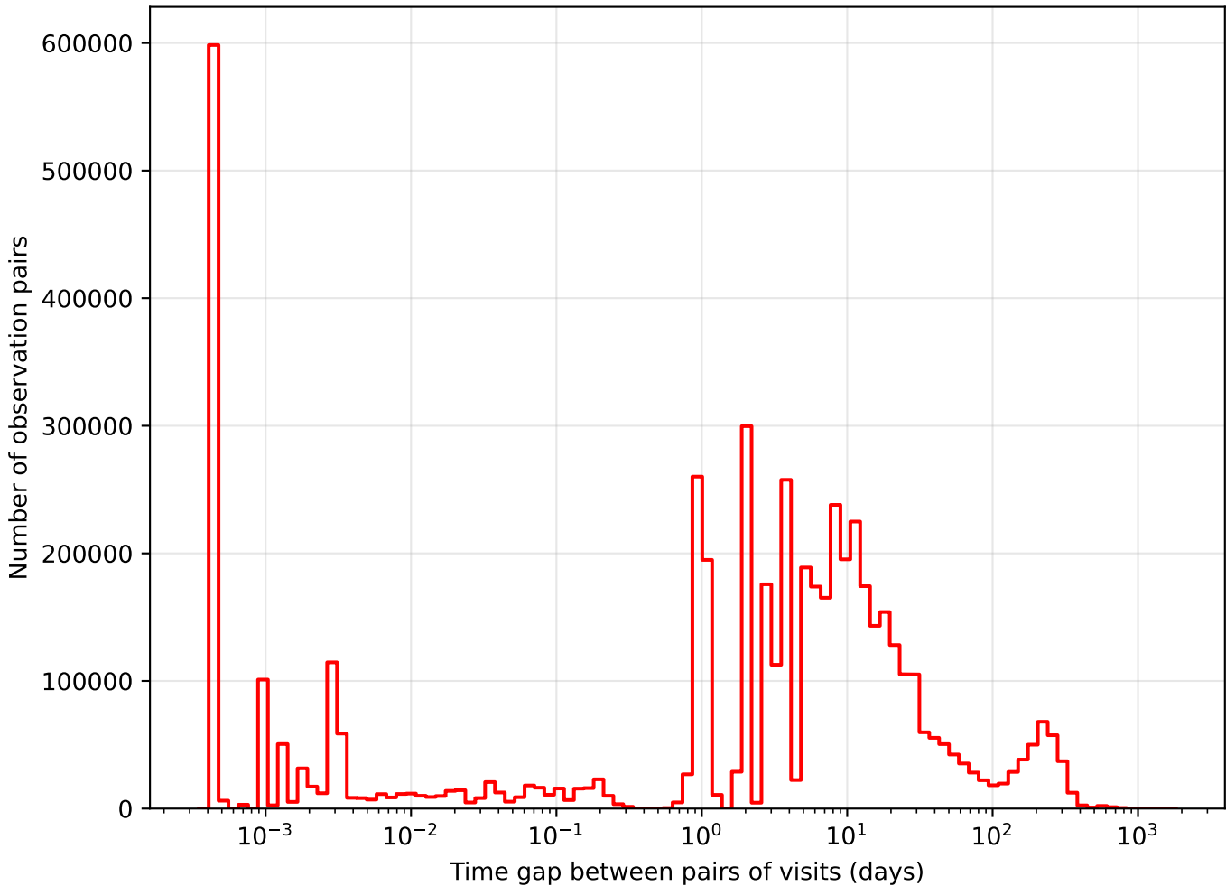
too_elab_r256_d3_griz_v3.4_10yrs i band: Tgaps observationStartMJD
