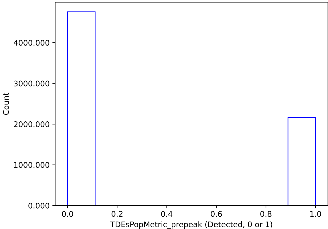
too_elab_r256_d3_griz_v3.4_10yrs : TDEsPopMetric_prepeak
