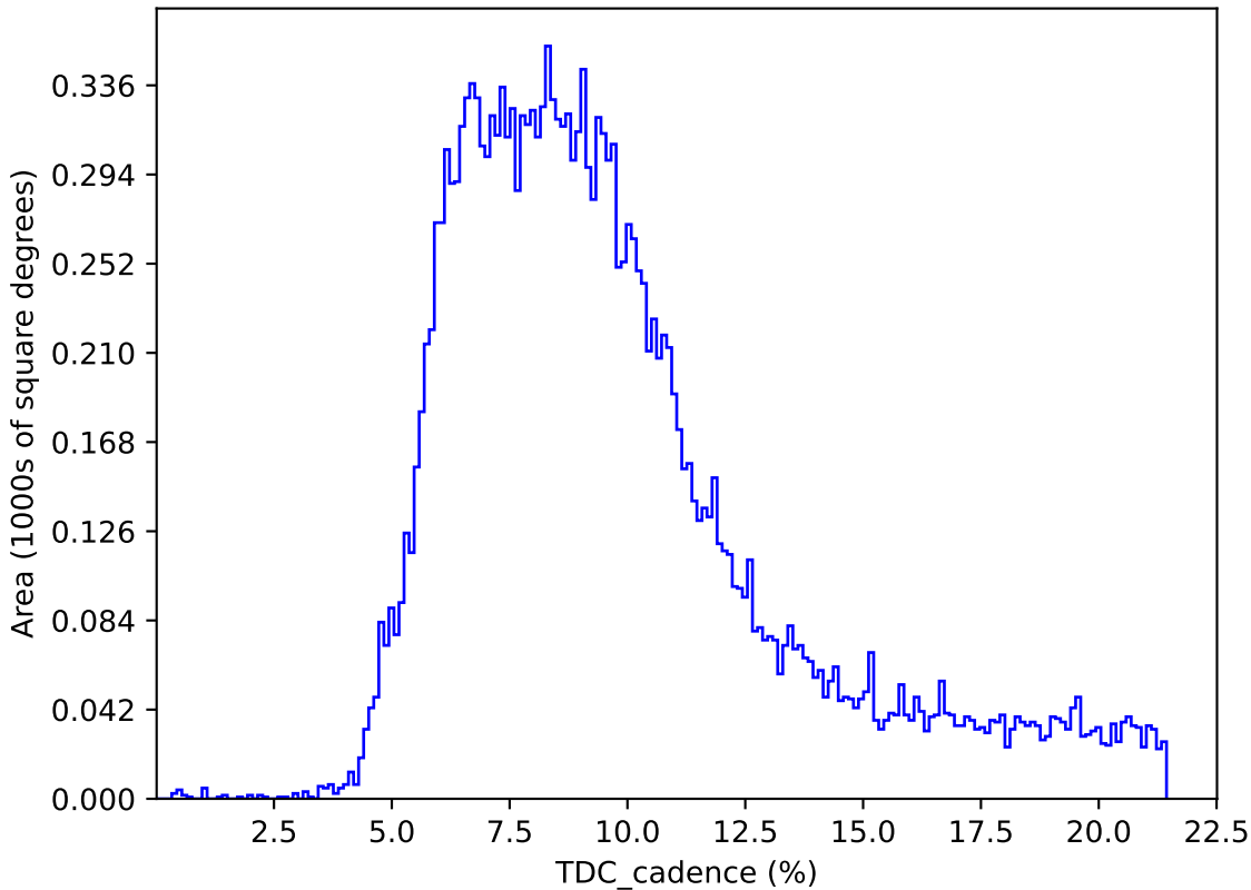
too_elab_r256_d3_griz_v3.4_10yrs : TDC_cadence
