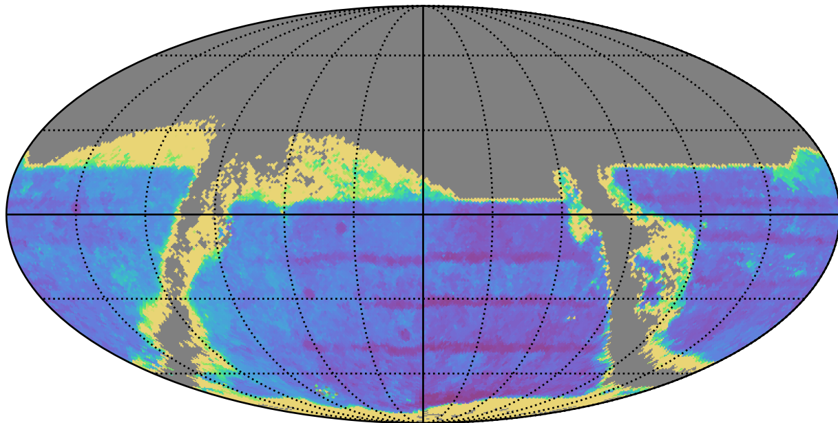
too_elab_r256_d3_griz_v3.4_10yrs : TDC_accuracy
