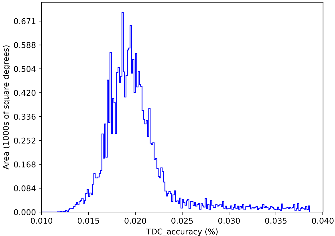
too_elab_r256_d3_griz_v3.4_10yrs : TDC_accuracy
