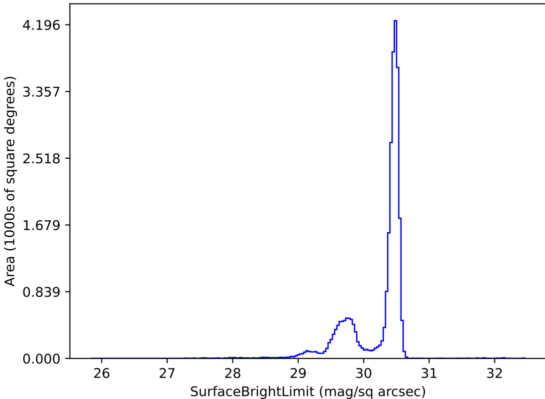
too_elab_r256_d3_griz_v3.4_10yrs r: SurfaceBrightLimit
