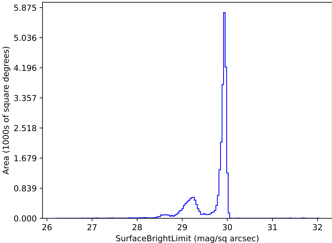
too_elab_r256_d3_griz_v3.4_10yrs i: SurfaceBrightLimit
