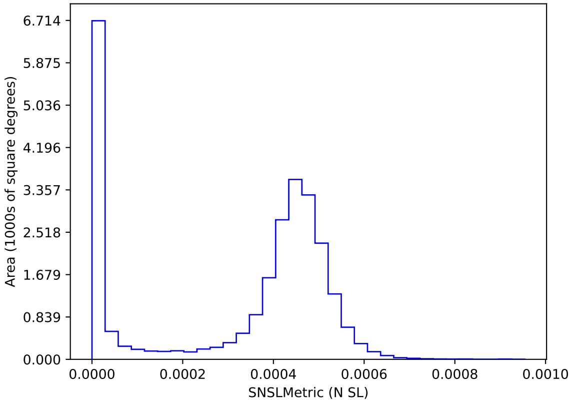
too_elab_r256_d3_griz_v3.4_10yrs : SNSLMetric
