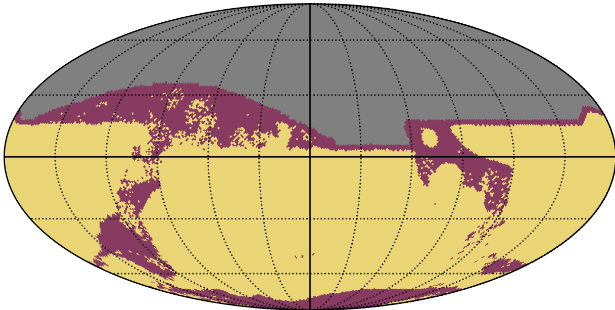
too_elab_r256_d3_griz_v3.4_10yrs : RapidRevisits
