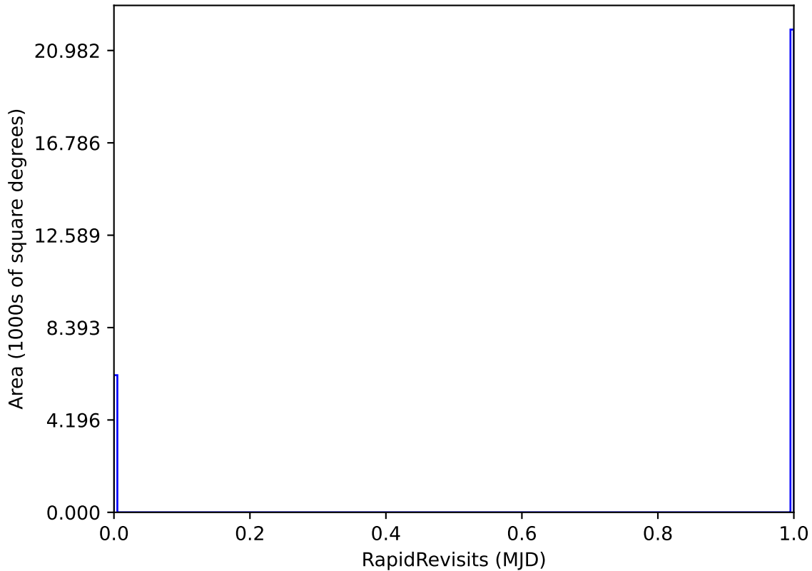
too_elab_r256_d3_griz_v3.4_10yrs : RapidRevisits
