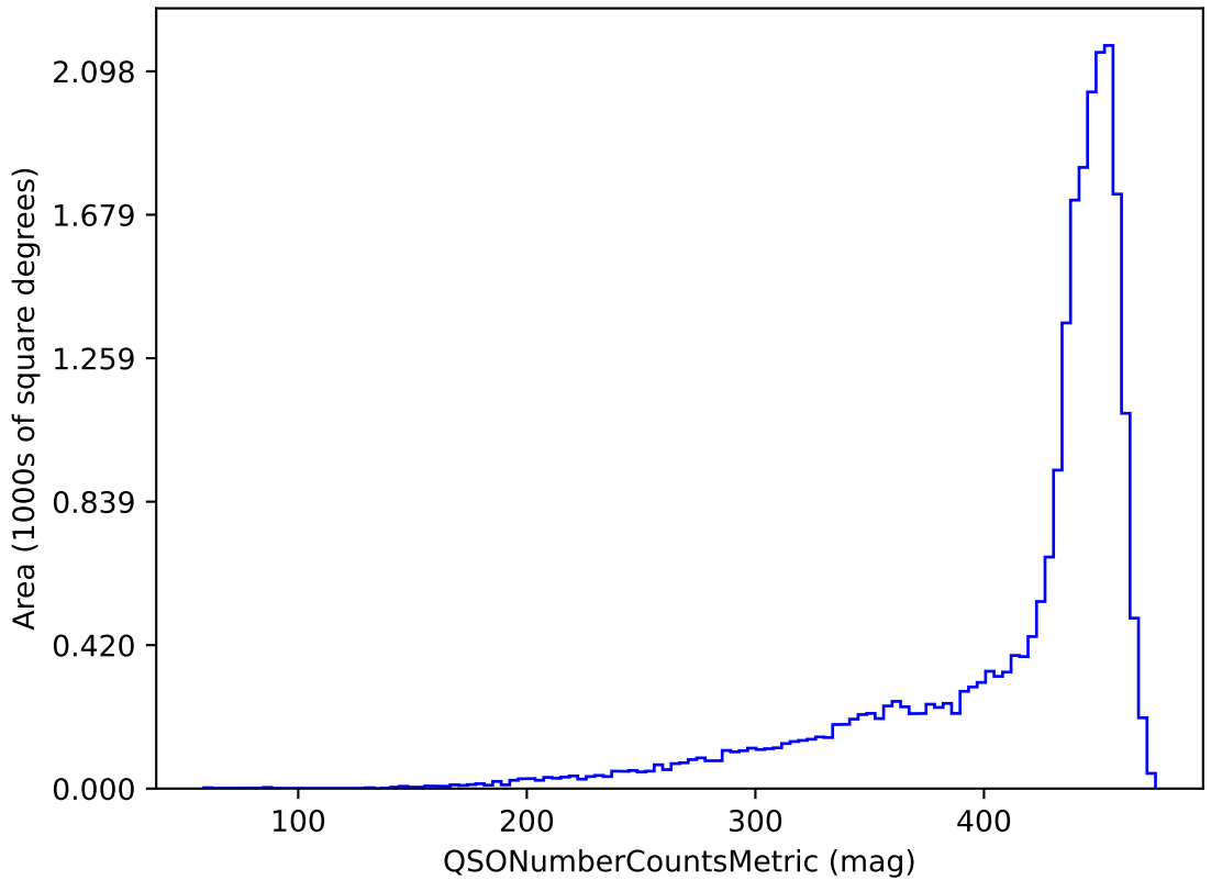
too_elab_r256_d3_griz_v3.4_10yrs g band and non-DD: QSONumberCountsMetric
