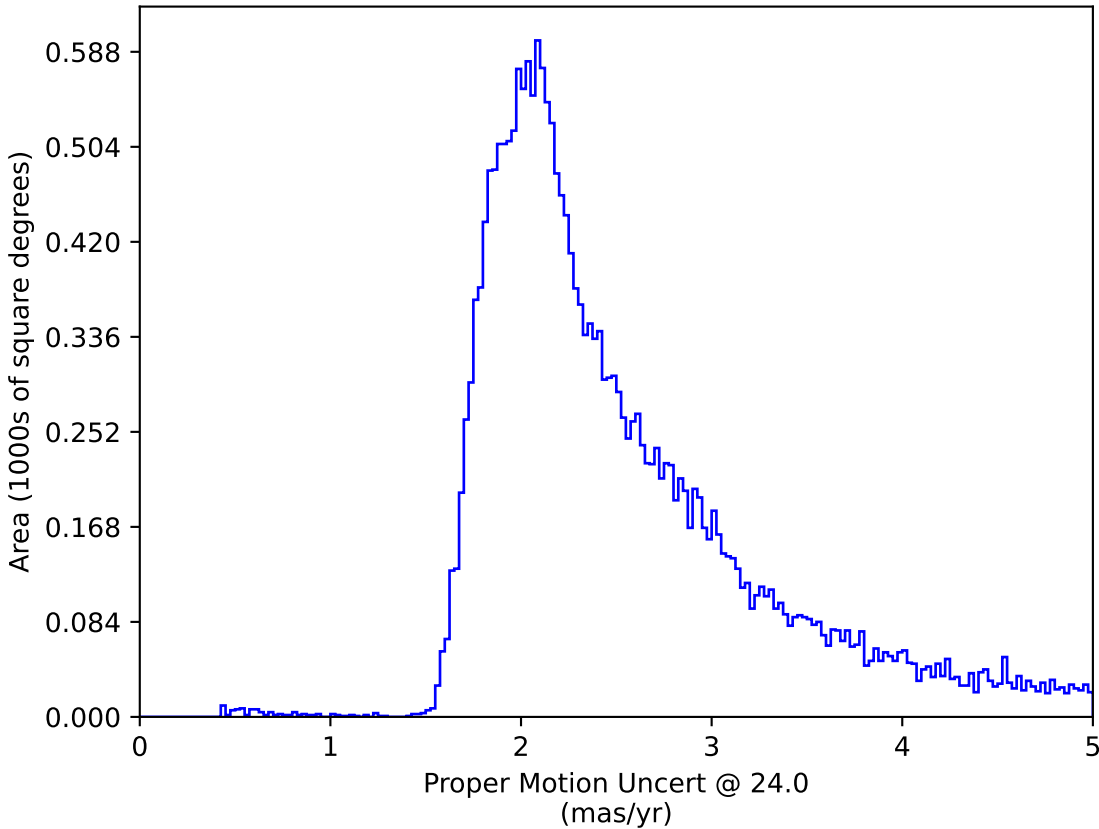
too_elab_r256_d3_griz_v3.4_10yrs : Proper Motion Uncert @ 24.0
