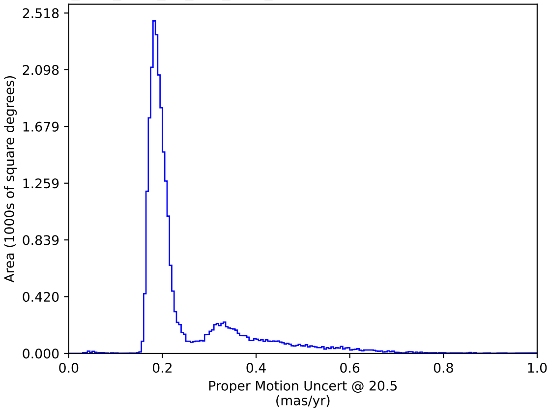
too_elab_r256_d3_griz_v3.4_10yrs : Proper Motion Uncert @ 20.5
