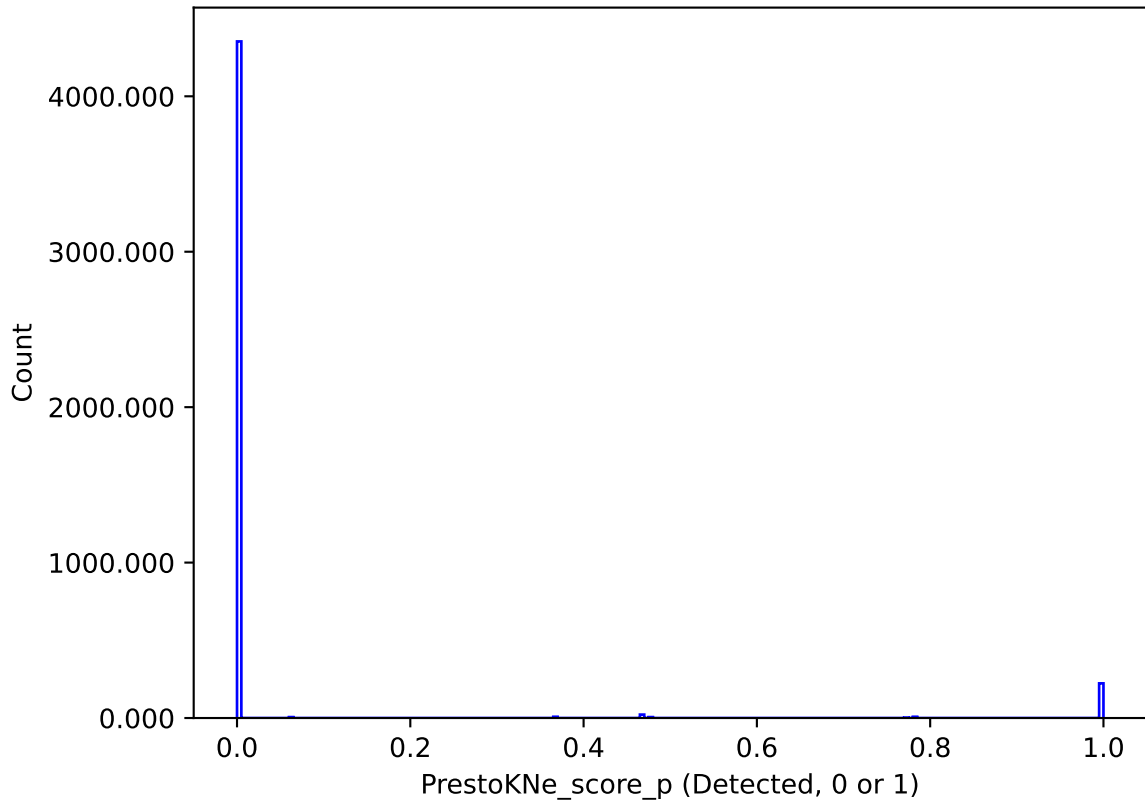
too_elab_r256_d3_griz_v3.4_10yrs : PrestoKNe_score_p
