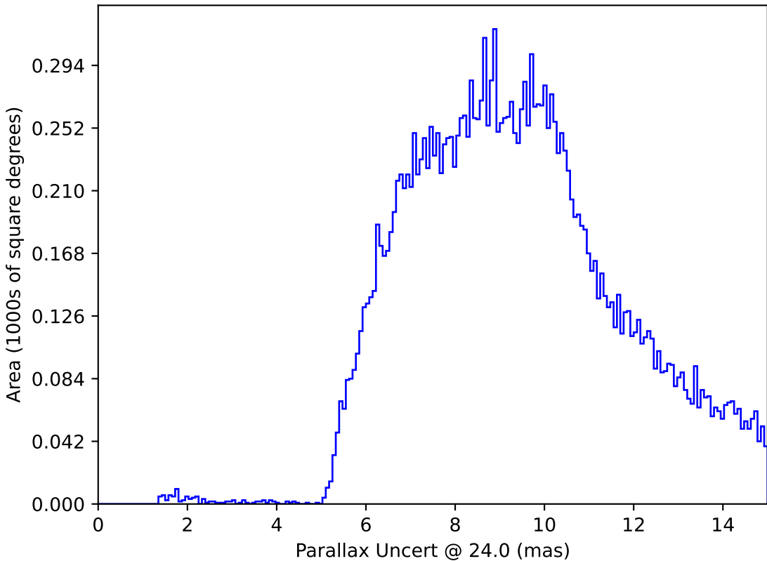
too_elab_r256_d3_griz_v3.4_10yrs : Parallax Uncert @ 24.0
