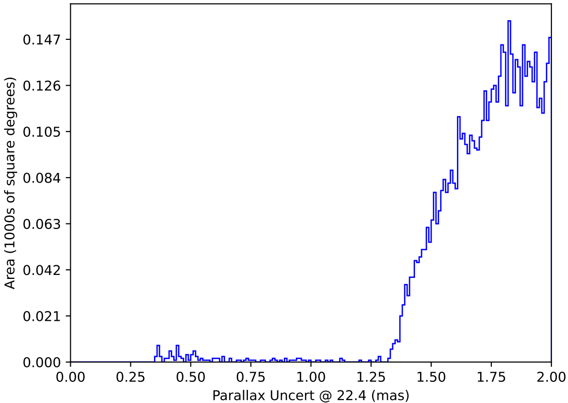
too_elab_r256_d3_griz_v3.4_10yrs : Parallax Uncert @ 22.4
