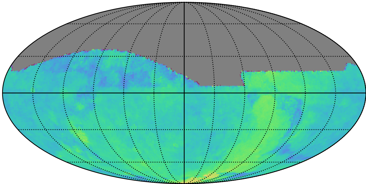
too_elab_r256_d3_griz_v3.4_10yrs : Parallax Coverage @ 22.4
