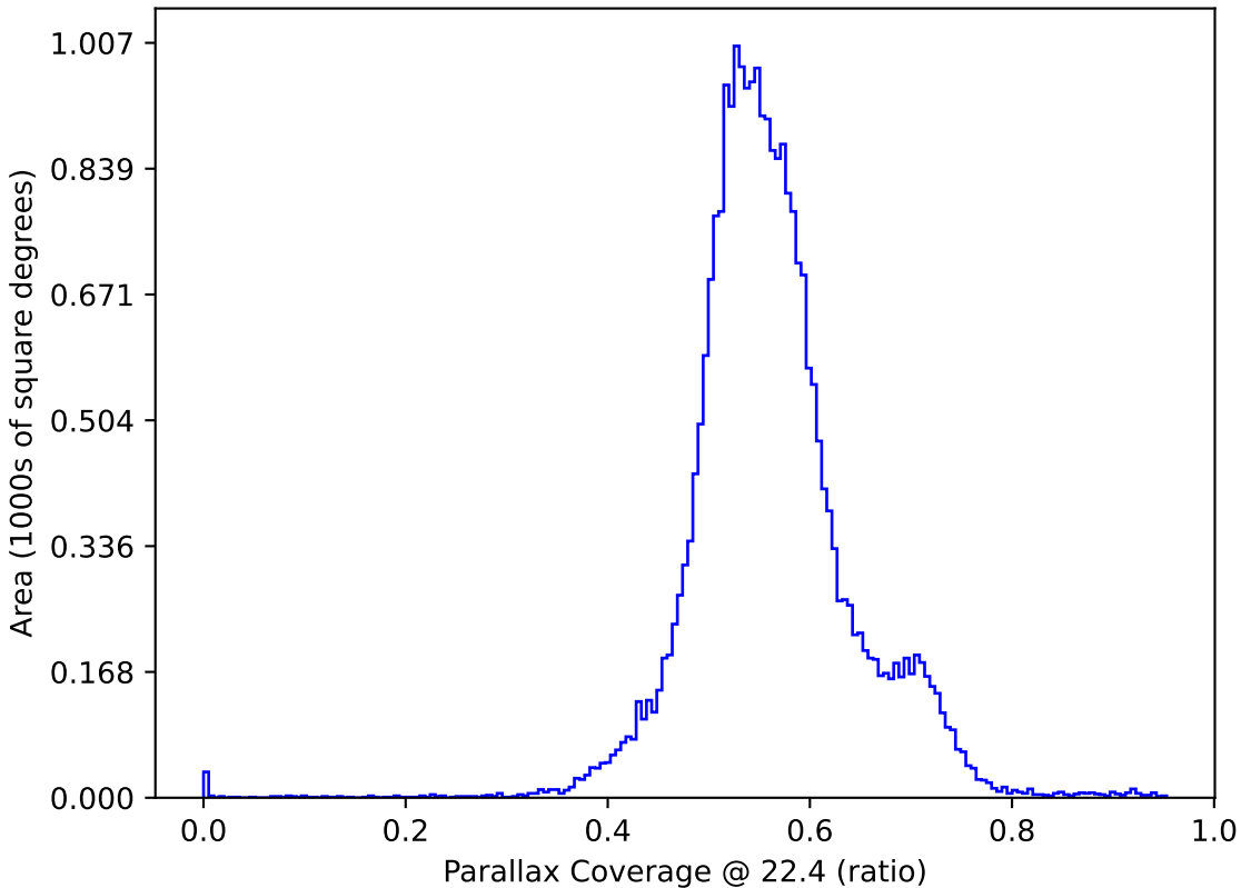
too_elab_r256_d3_griz_v3.4_10yrs : Parallax Coverage @ 22.4
