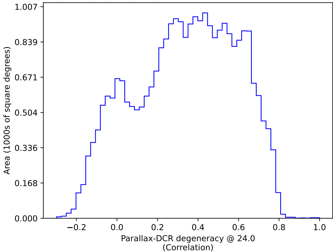
too_elab_r256_d3_griz_v3.4_10yrs : Parallax-DCR degeneracy @ 24.0
