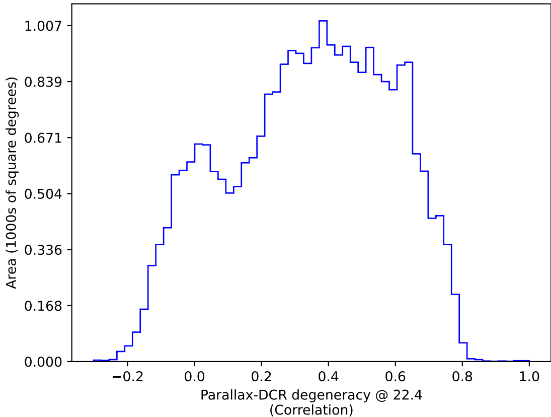
too_elab_r256_d3_griz_v3.4_10yrs : Parallax-DCR degeneracy @ 22.4
