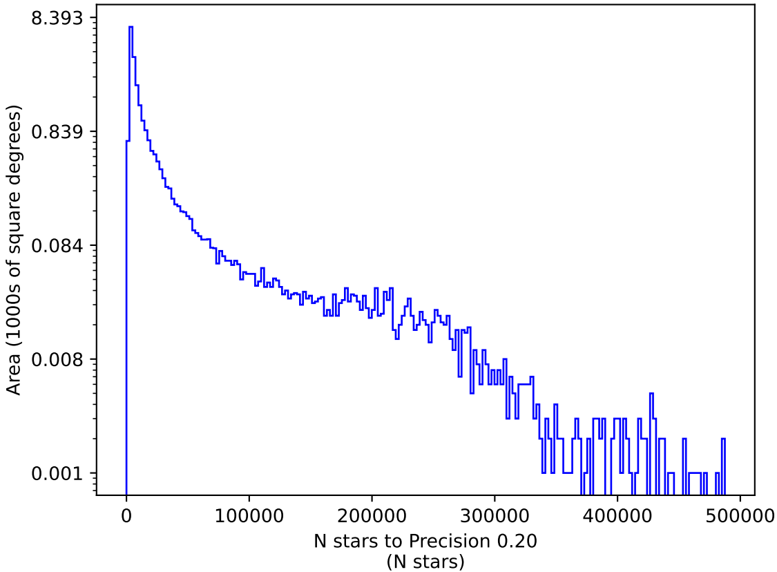
too_elab_r256_d3_griz_v3.4_10yrs u: N stars to Precision 0.20
