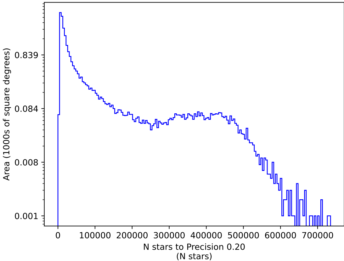
too_elab_r256_d3_griz_v3.4_10yrs r: N stars to Precision 0.20
