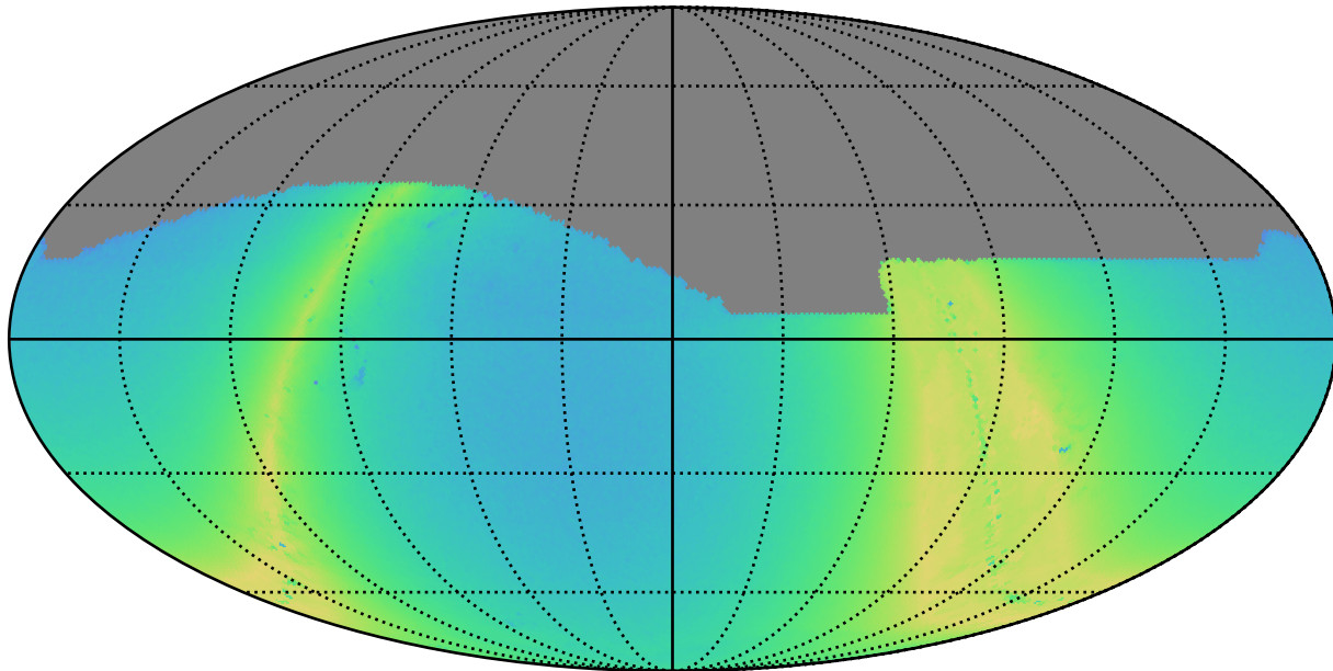
too_elab_r256_d3_griz_v3.4_10yrs i: N stars to Precision 0.20
