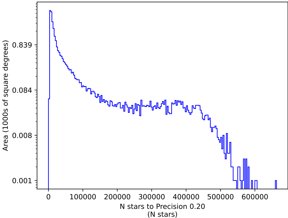
too_elab_r256_d3_griz_v3.4_10yrs g: N stars to Precision 0.20
