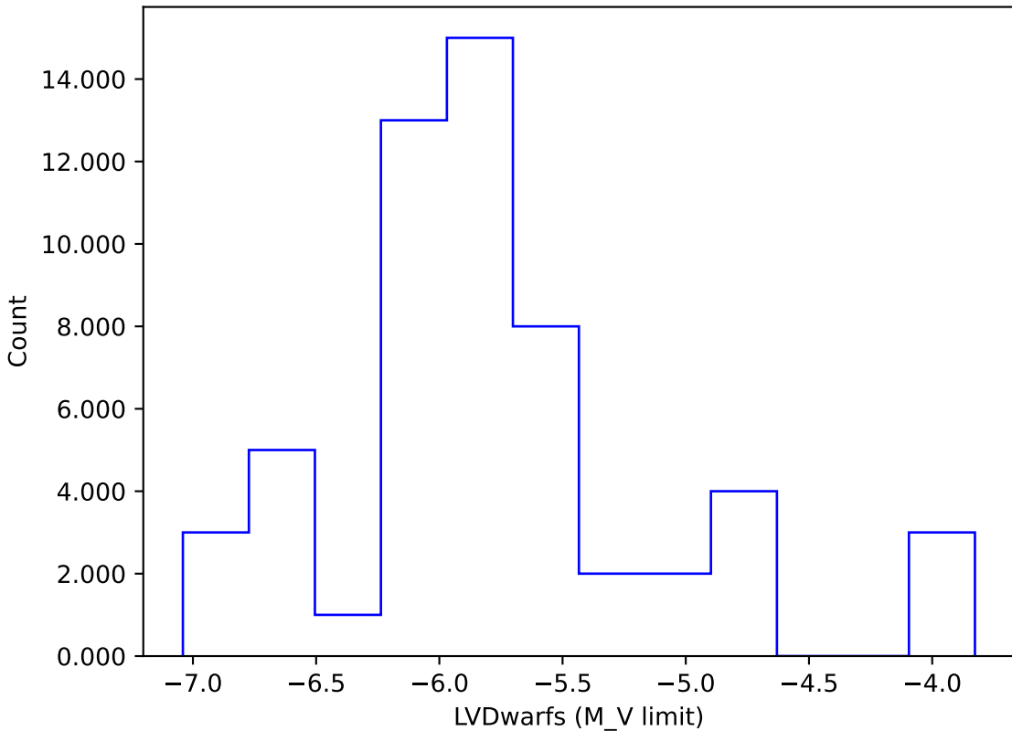
too_elab_r256_d3_griz_v3.4_10yrs gi: LVDwarfs
