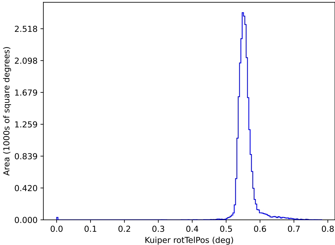
too_elab_r256_d3_griz_v3.4_10yrs y: Kuiper rotTelPos
