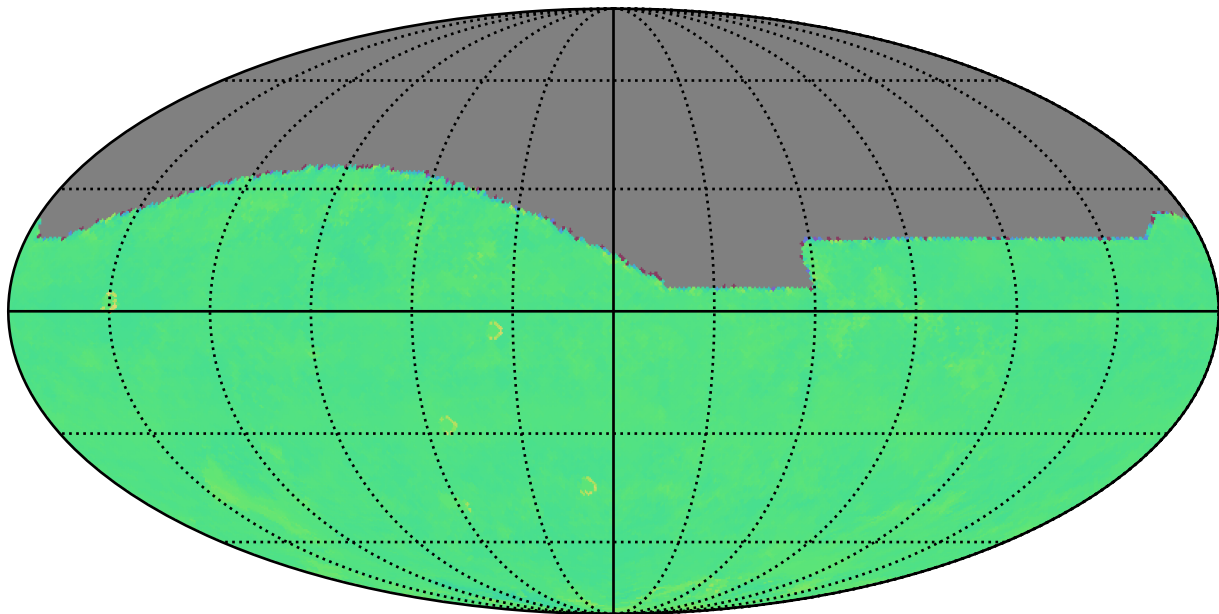
too_elab_r256_d3_griz_v3.4_10yrs r: Kuiper rotTelPos
