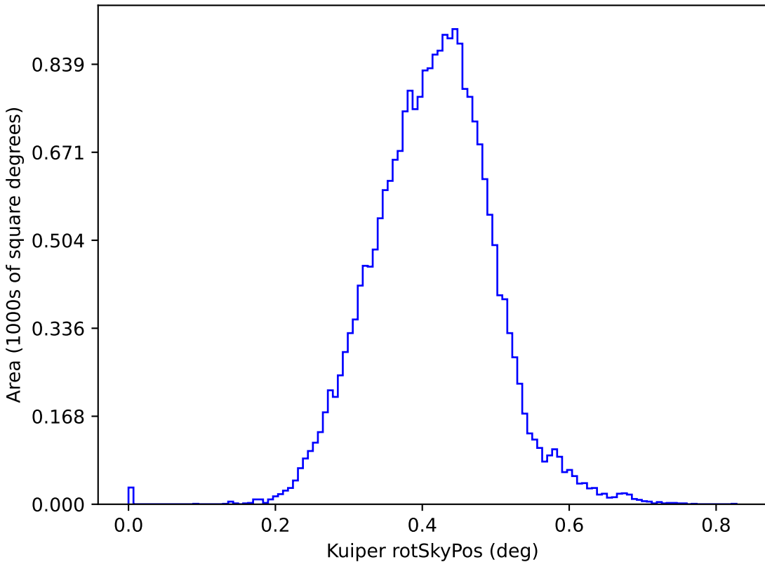
too_elab_r256_d3_griz_v3.4_10yrs y: Kuiper rotSkyPos
