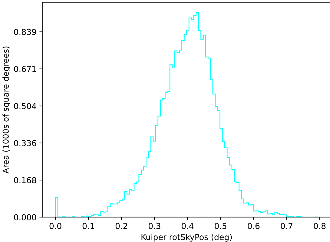
too_elab_r256_d3_griz_v3.4_10yrs u: Kuiper rotSkyPos
