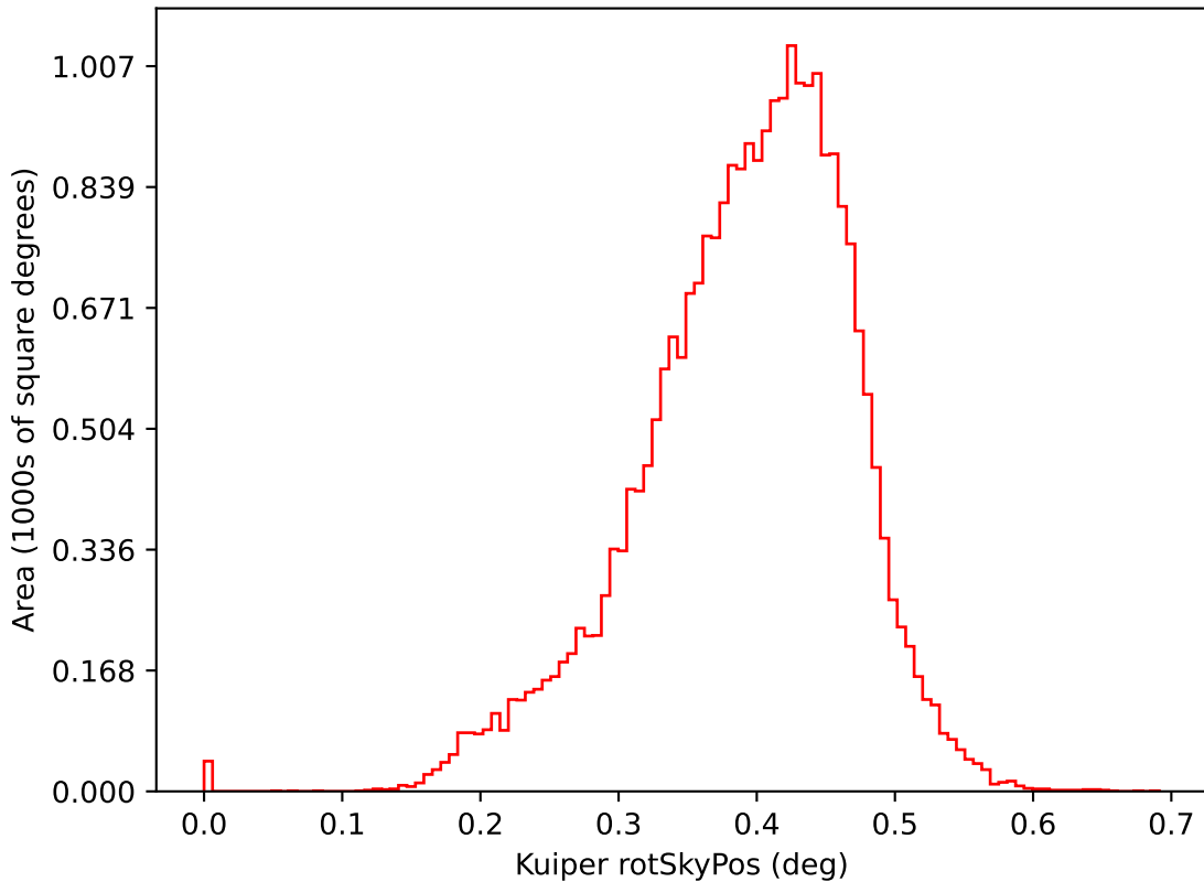
too_elab_r256_d3_griz_v3.4_10yrs i: Kuiper rotSkyPos
