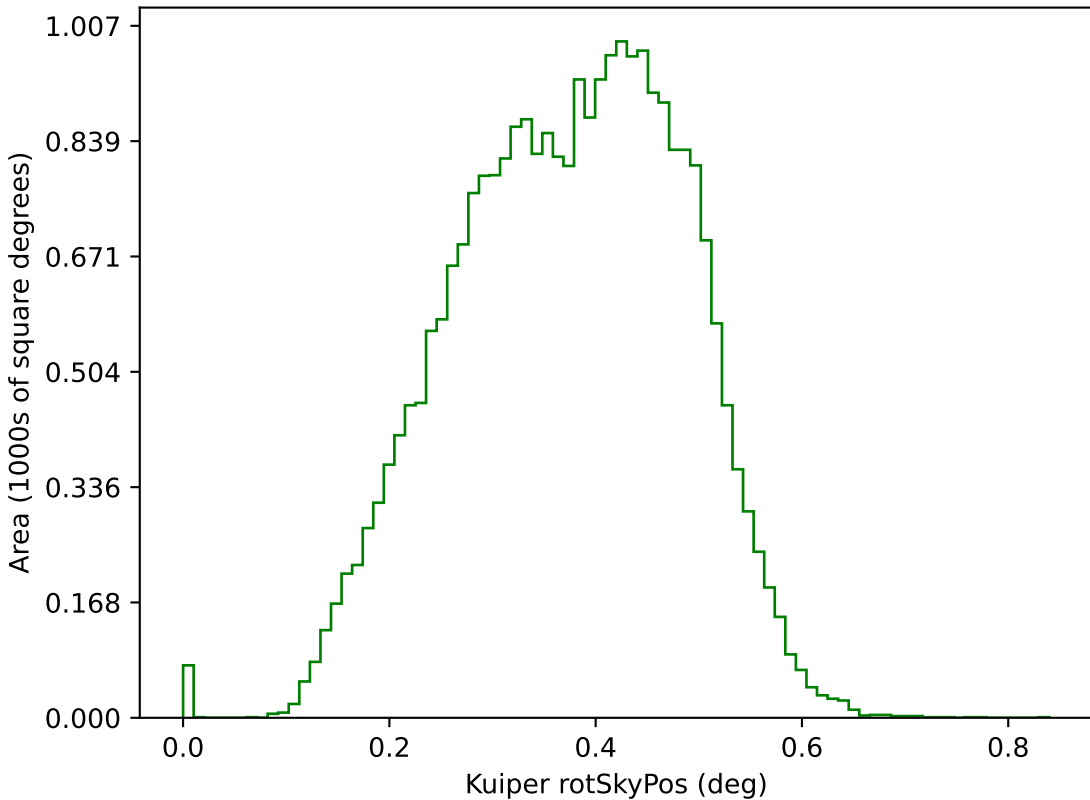
too_elab_r256_d3_griz_v3.4_10yrs g: Kuiper rotSkyPos
