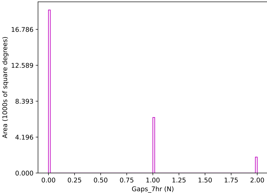
too_elab_r256_d3_griz_v3.4_10yrs z band: Gaps_7hr
