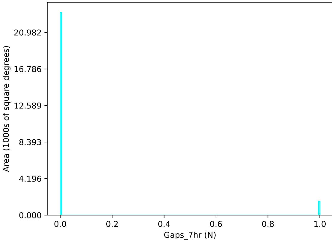
too_elab_r256_d3_griz_v3.4_10yrs u band: Gaps_7hr
