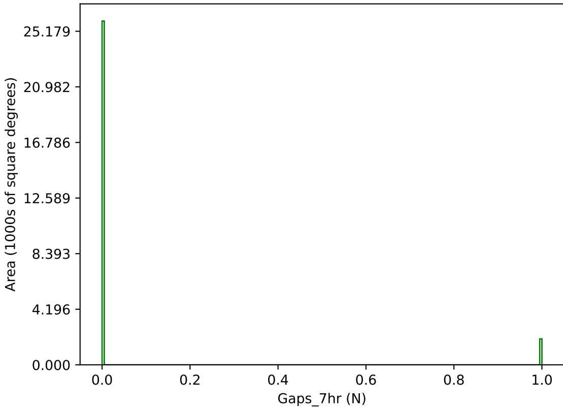
too_elab_r256_d3_griz_v3.4_10yrs g band: Gaps_7hr
