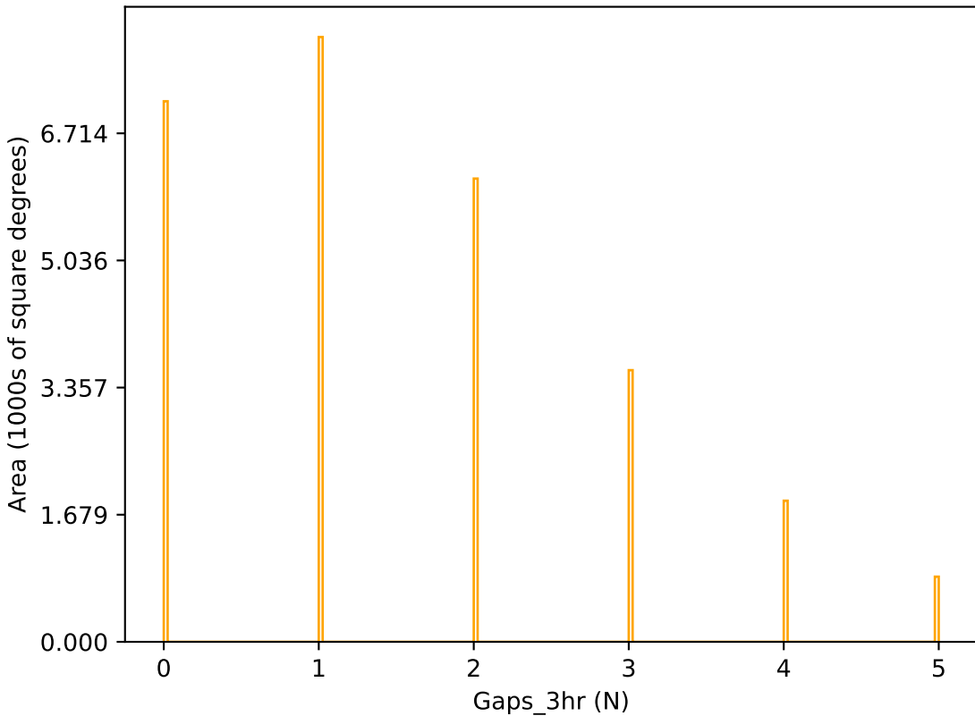
too_elab_r256_d3_griz_v3.4_10yrs r band: Gaps_3hr
