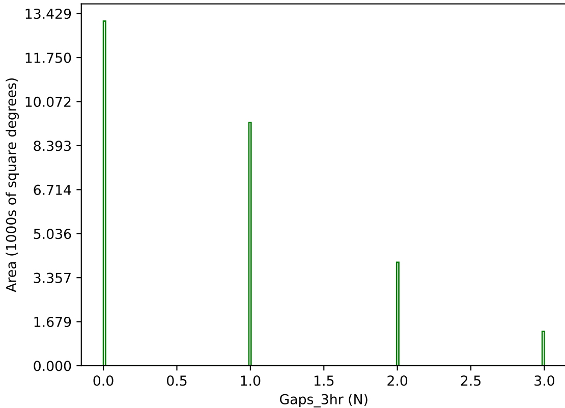
too_elab_r256_d3_griz_v3.4_10yrs g band: Gaps_3hr
