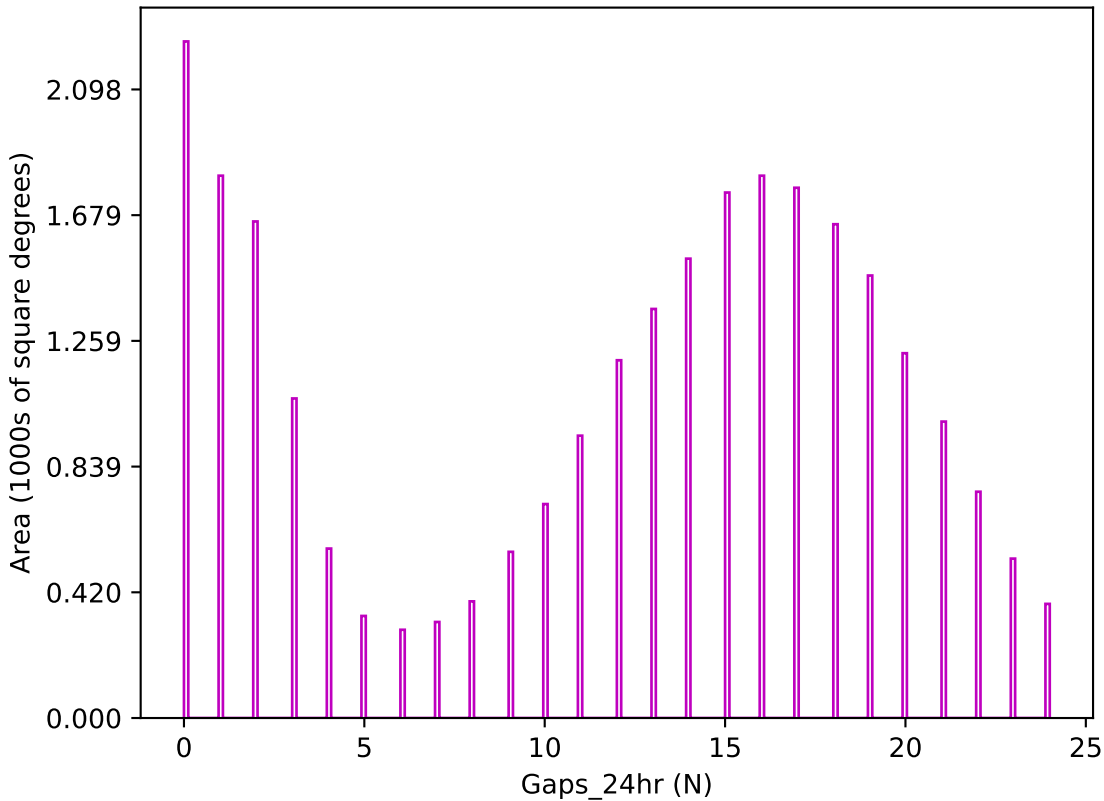
too_elab_r256_d3_griz_v3.4_10yrs z band: Gaps_24hr
