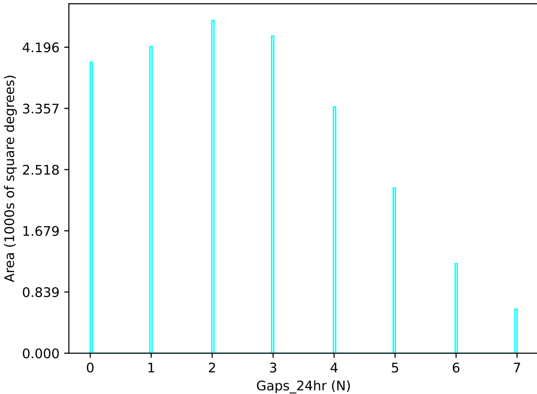
too_elab_r256_d3_griz_v3.4_10yrs u band: Gaps_24hr
