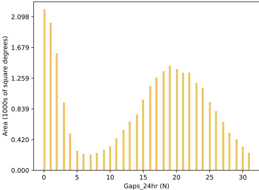
too_elab_r256_d3_griz_v3.4_10yrs r band: Gaps_24hr
