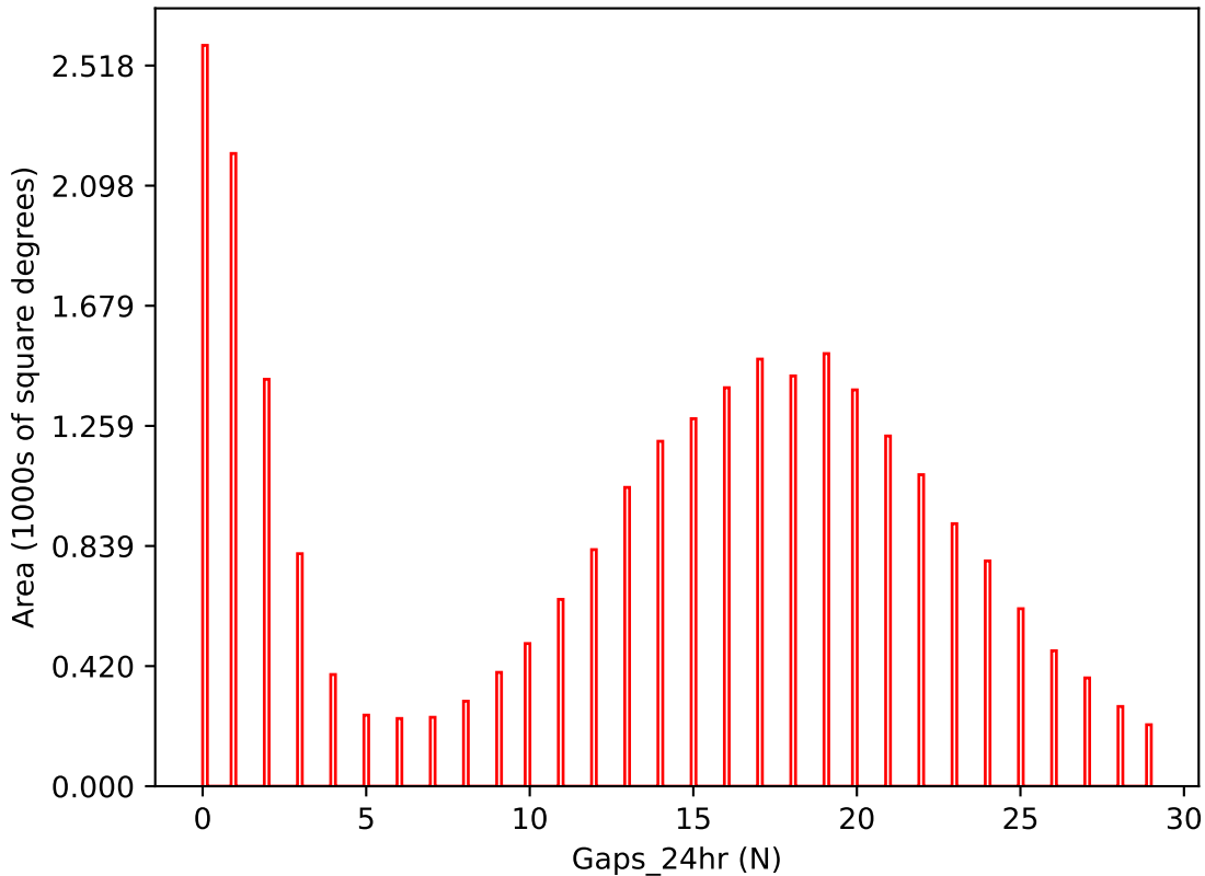
too_elab_r256_d3_griz_v3.4_10yrs i band: Gaps_24hr
