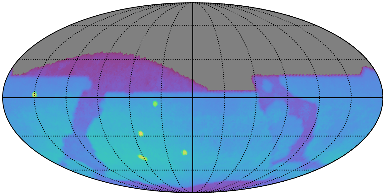
too_elab_r256_d3_griz_v3.4_10yrs : Brown Dwarf, L7
