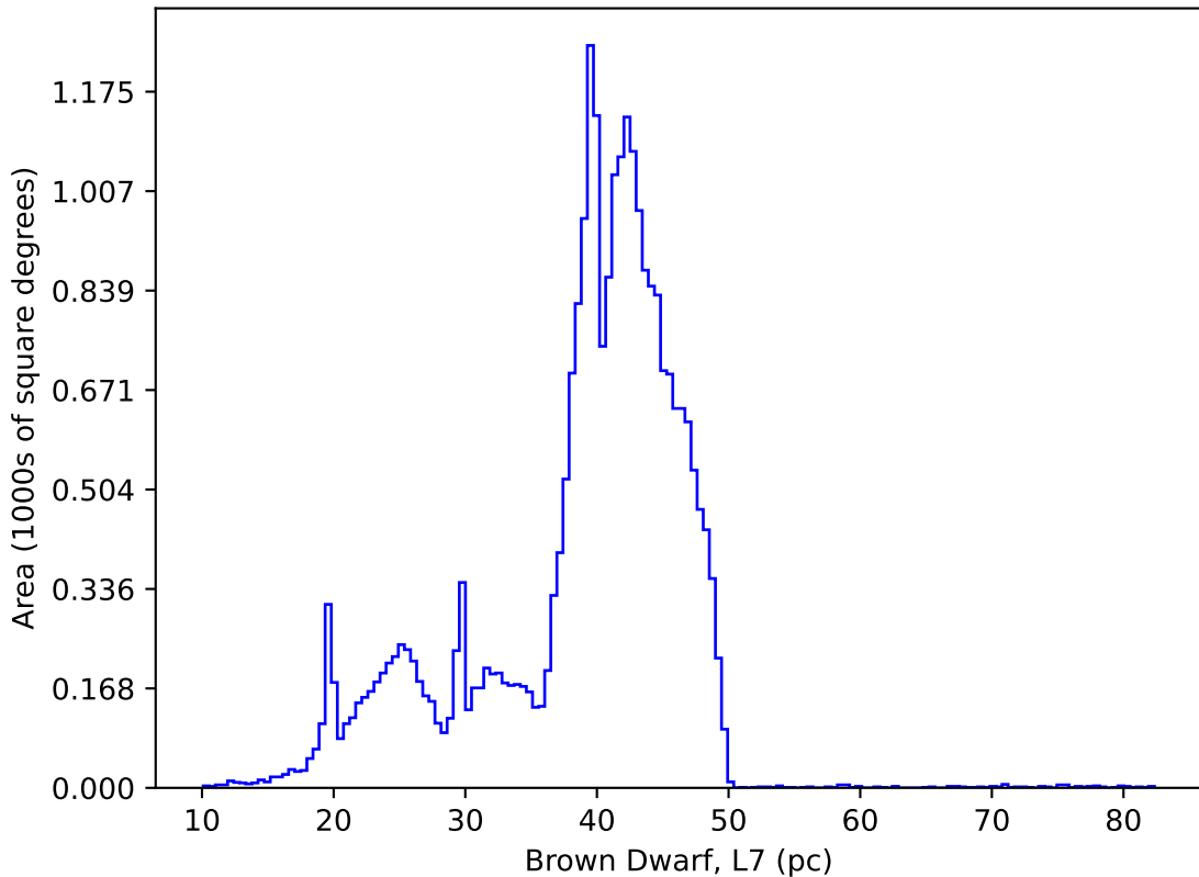
too_elab_r256_d3_griz_v3.4_10yrs : Brown Dwarf, L7
