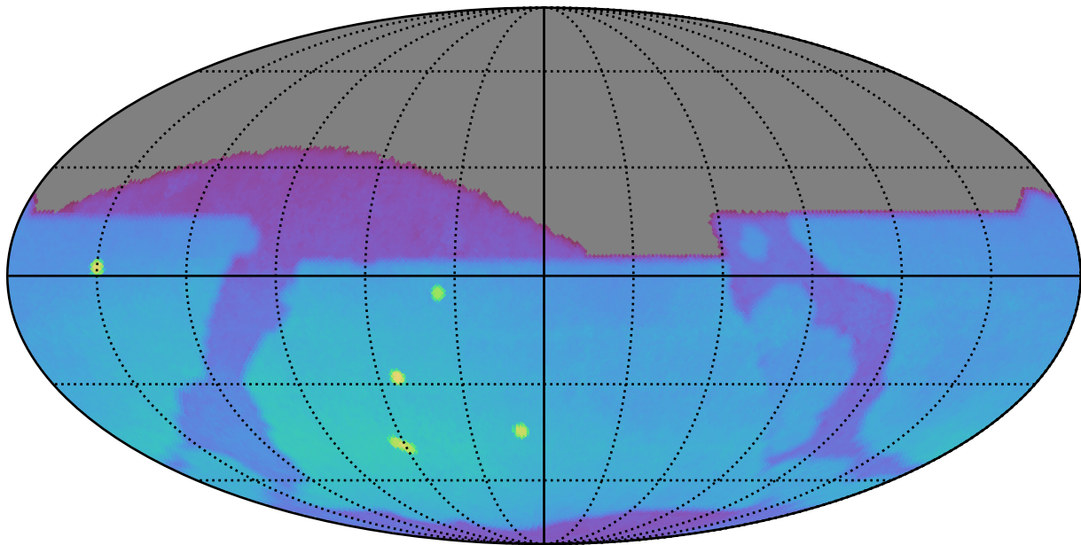
too_elab_r256_d3_griz_v3.4_10yrs : Brown Dwarf, L4
